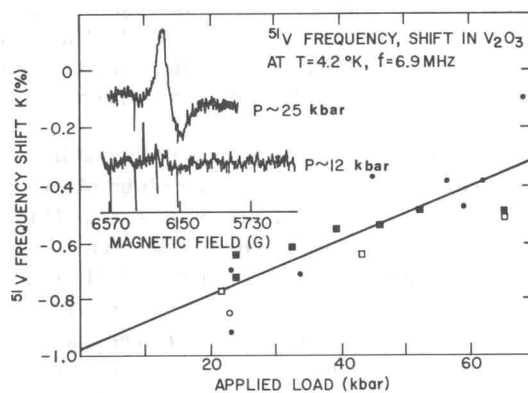
FIG. 2. ^{51}\text{V} frequency shifts in \text{V}_2\text{O}_3 at T=4.2 °K and f=6.9 MHz. Circles and squares refer to measurements taken, respectively, on the initial application of load and on a second application of load two days later. Closed data points refer to measurements made with increasing load and open data points to measurements with decreasing load. A later measurement on a third sample using spin-echo amplitude measurements at 26 kbar gave K(26 \text{ kbar}) = -0.92\% \pm 0.20\% . The calibration of the load was obtained from the 25.5-kbar transition of bismuth on the initial loading, as described in the text. During the second loading (square data points) it was noted that the bismuth transition was reached under \sim 20\% less load than on the initial loading. For this reason, the pressure on the \text{V}_2\text{O}_3 sample in the 20- to 30-kbar regime is as much as 5 kbar greater than indicated for the square points. Conversely, in the regime above 50 kbar, cracking of the girdle may have resulted in a reduction of pressure. Correction for these two effects would raise the already anomalously high slope shown for the frequency shift versus pressure. It is also probable that in the presence of pressure inhomogeneities in the 20- to 30-kbar regime the portions of the sample in the higher-pressure regions would contribute more strongly to the observed resonance than would those portions of sample in lower-pressure regions. This phenomenon would result from the rapid falloff in resonance intensity at low pressures demonstrated in Fig. 3 and in the inset of this figure. For this reason, also, the data points in the 20- to 30-kbar regime may represent pressures up to 5 kbar greater than shown. Consideration of such a correction would also increase the frequency-shift-versus-pressure slope. The inset of the figure shows free-induction-decay nuclear-resonance amplitudes as measured with phase-coherent detection at 25 and 12 kbar. The greatly reduced amplitude at 12 kbar results from the fact that the sample is antiferromagnetically ordered at this pressure, and the nuclear resonance is consequently shifted out of the region of observability to a much higher frequency.
